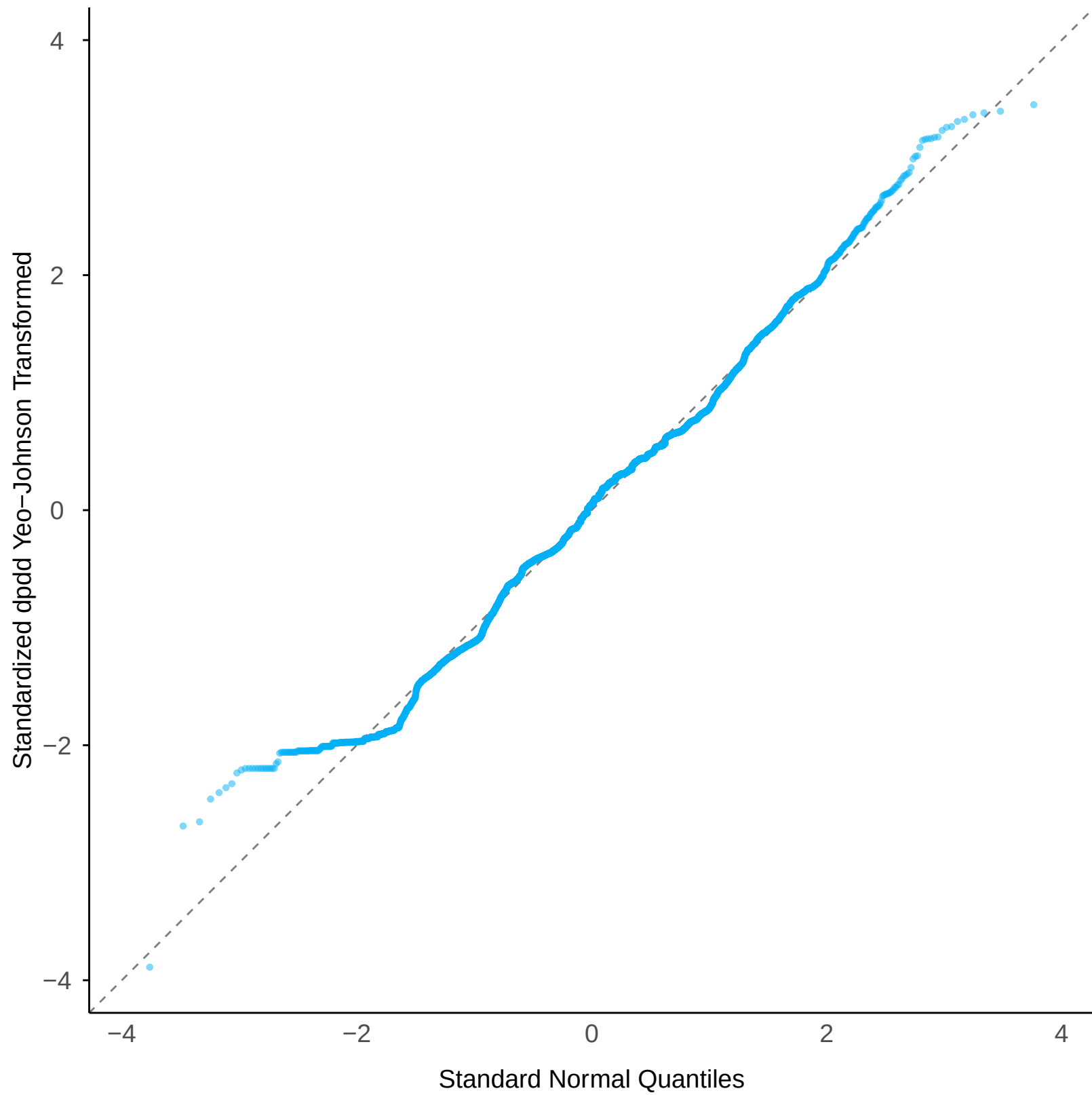
Normal Q-Q: dpdd Yeo-Johnson Transformed
